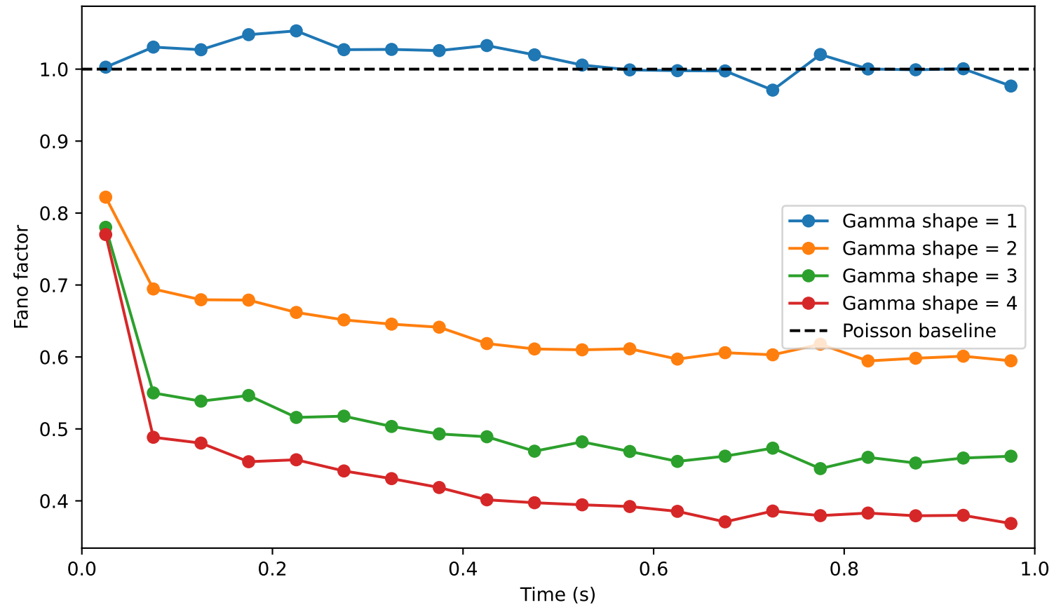
Fano factor for ramp model: \beta = 1.1 , \sigma = 0.3
